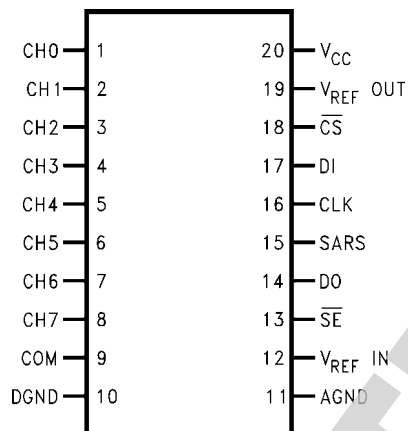
ADC08138CIWM Small Outline Packages
