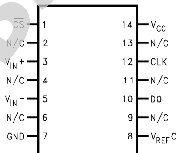
ADC08131CIWM Small Outline Package
