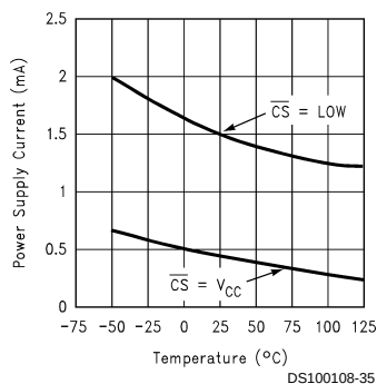
Power Supply Current vs Temperature (ADC08831)
