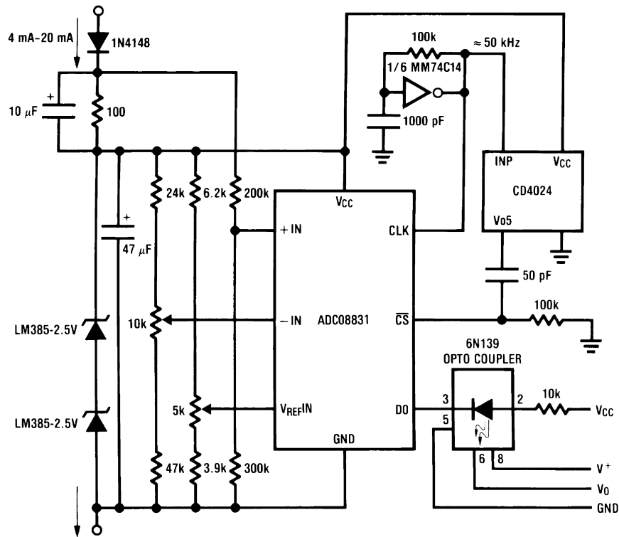
4 mA-20 mA Current Loop Converter
