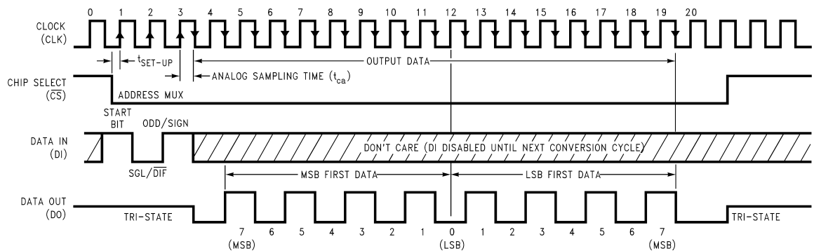
ADC08832 Timing
