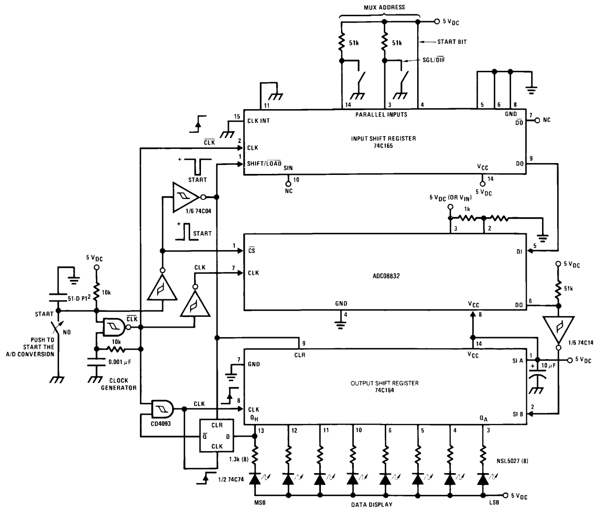
A "Stand-Alone" Hook-Up for ADC08832 Evaluation
