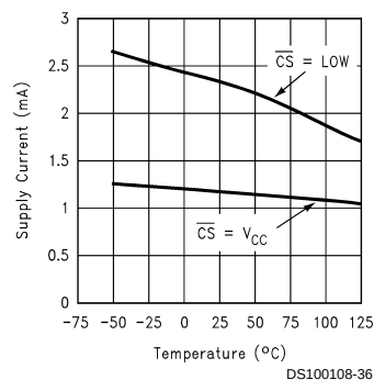
Power Supply Current vs Temperature (ADC08832)
