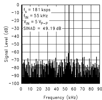
Spectral Response with 55 KHz Sine Wave Input
