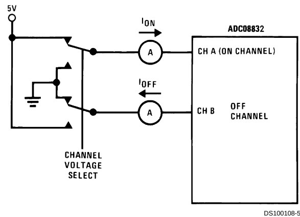
Leakage Current Test Circuit
