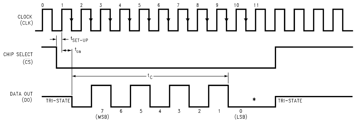
ADC08831 Timing
