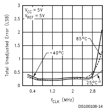
Linearity Error (TUE) vs Clock Frequency
