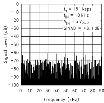
Spectral Response with 10KHz Sine Wave Input
