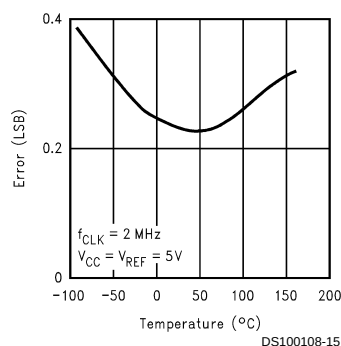
Linearity Error (TUE) vs Temperature
