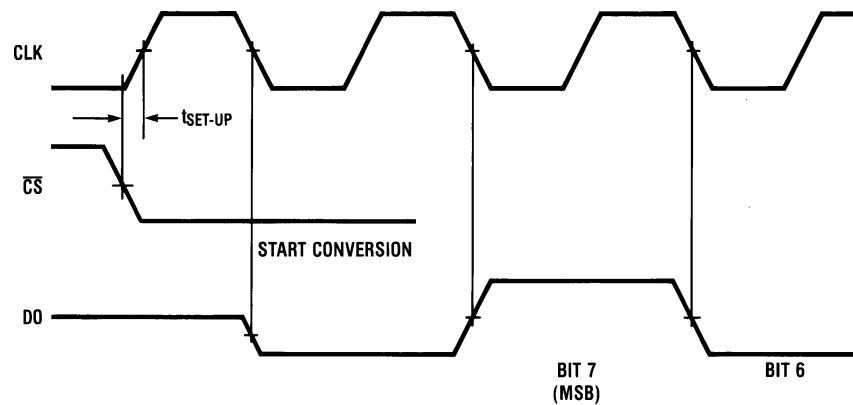
ADC08831 Start Conversion Timing
