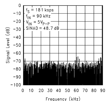
Spectral Response with 90 KHz Sine Wave Input
