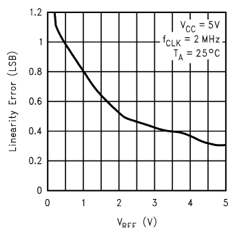
Linearity Error (TUE) vs Reference Voltage
