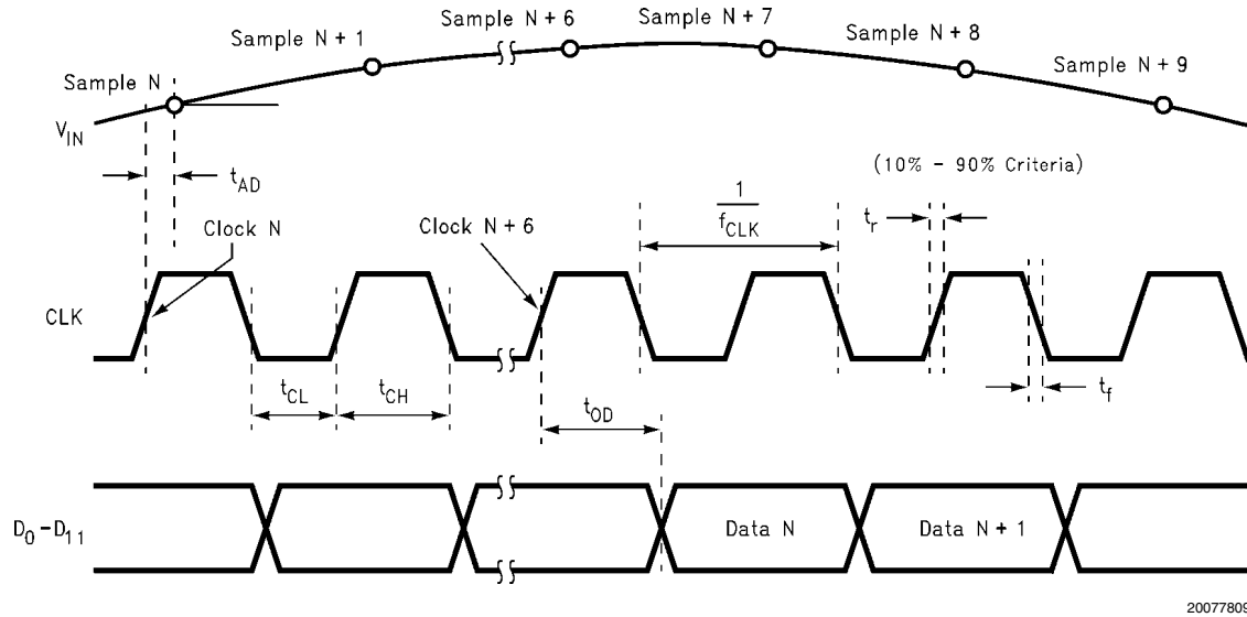
FIGURE 1. Clock and Data Timing Diagram
