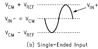
FIGURE 2. Expected Input Signal Range
