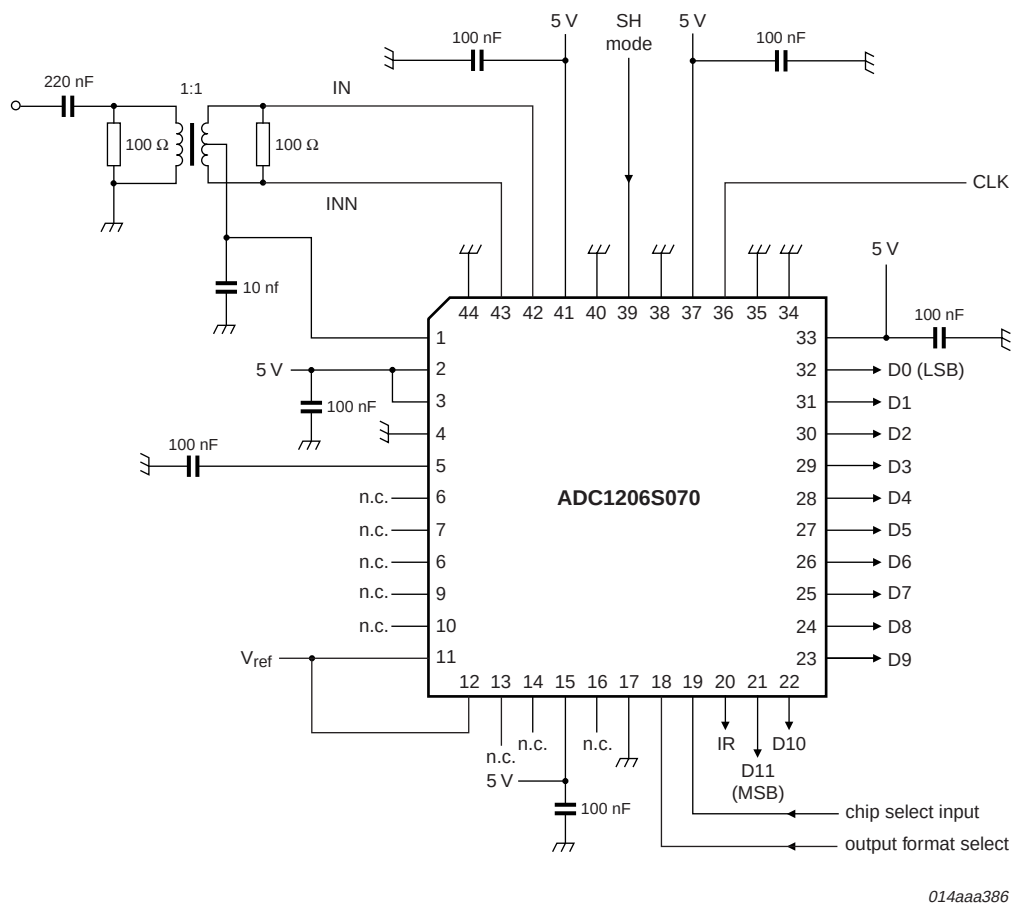
Fig 17. Application diagram
