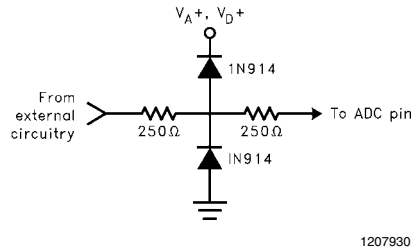
FIGURE 6. Protecting the MUXOUT1, MUXOUT2, A/DIN1 and A/DIN2 Analog Pins
