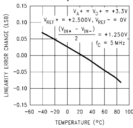
Linearity Error Change vs. Temperature
