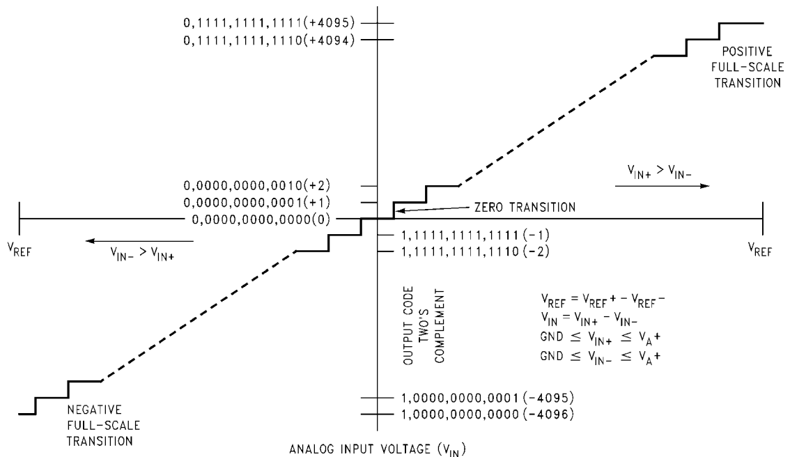
FIGURE 1. Transfer Characteristic
