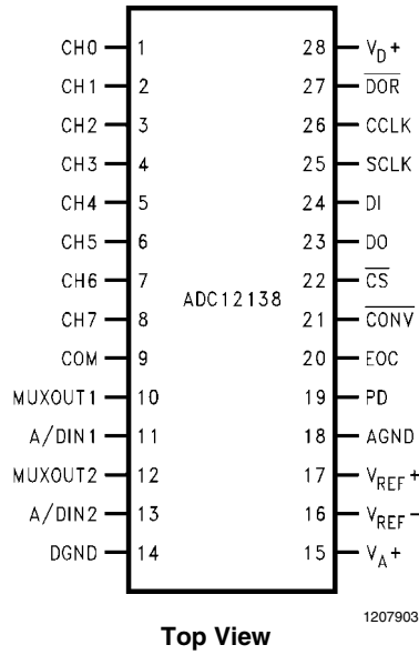
28-Pin Dual-In-Line, SSOP and Wide Body SO Packages
