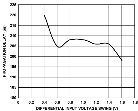
Figure 5. Propagation Delay vs. Differential Input Voltage
