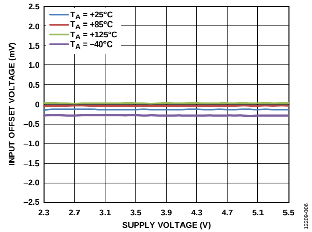
Figure 6. Input Offset Voltage ( V_{OS} ) vs. Supply Voltage ( V_{CC} ), V_{CM} = 1 V for Various Temperatures
