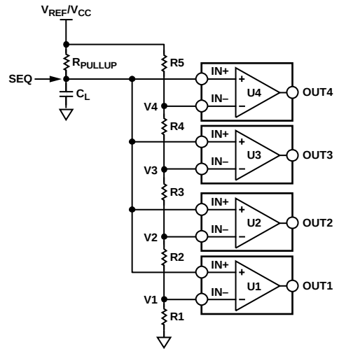
Figure 30. Programmable Sequencing Control Circuit
