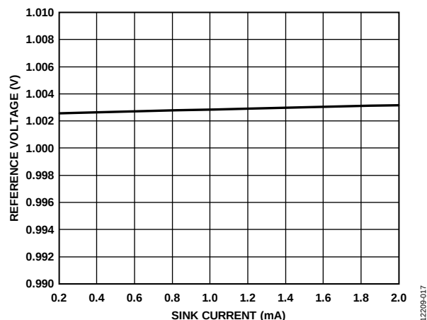
Figure 17. Reference Voltage ( V_{REF} ) vs. Sink Current ( I_{SINK} ) of the REF Pin, V_{CC} = 3.3 V
