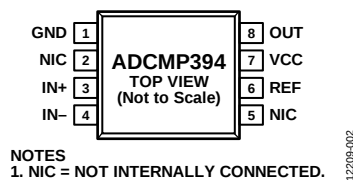
Figure 2. Pin Configuration
