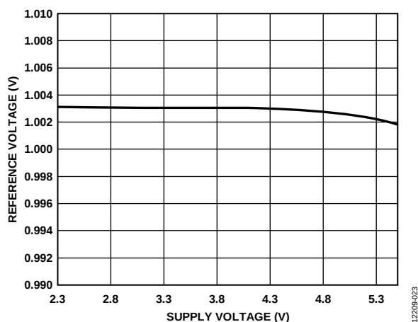
Figure 23. Reference Voltage ( V_{REF} ) vs. Supply Voltage ( V_{CC} )
