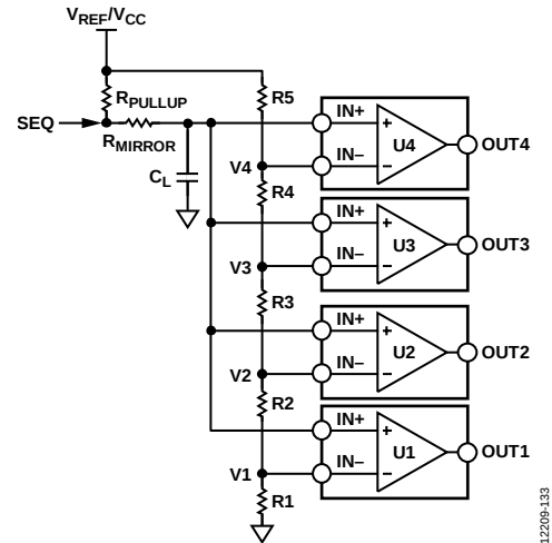
Figure 33. Circuit Configuration for a Mirrored Voltage Sequencer
