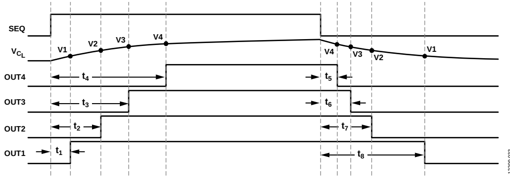
Figure 34. Mirrored Voltage Sequencer Timing Diagram
