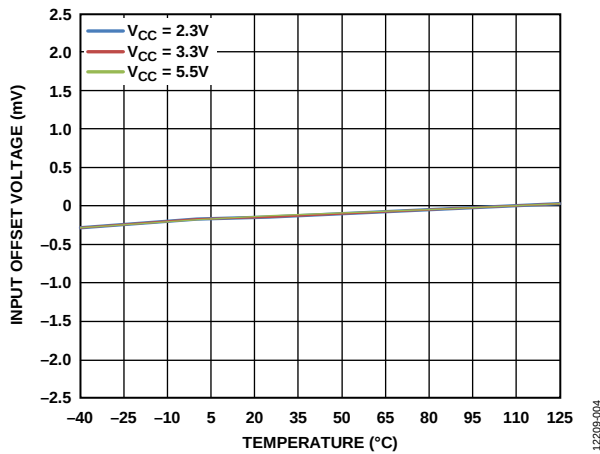
Figure 4. Input Offset Voltage ( V_{OS} ) vs. Temperature for Various Supply Voltages ( V_{CC} ), V_{CM} = 1 V
