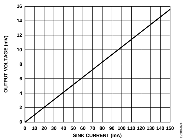
Figure 24. Output Voltage Low vs. Sink Current ( I_{SINK} ), V_{CC} = 0.9\text{ V}
