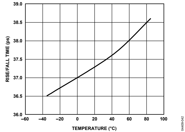
Figure 6. Rise/Fall Time vs. Temperature
