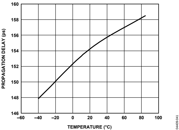
Figure 5. Propagation Delay vs. Temperature
