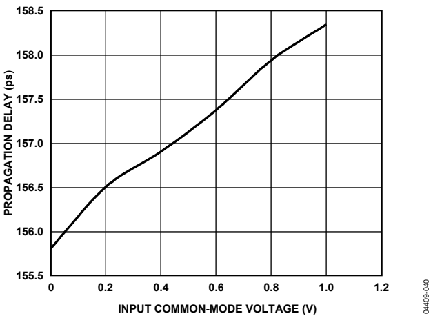
Figure 4. Propagation Delay vs. Input Common-Mode
