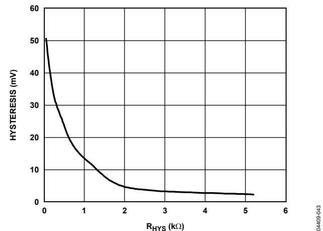
Figure 7. Hysteresis vs. R_{HYS} Control Resistor
