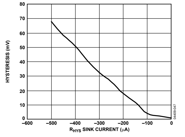
Figure 8. Hysteresis vs. R_{HYS} Sink Current
