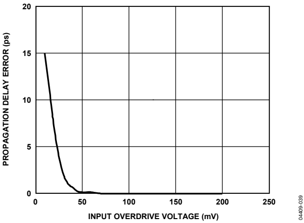
Figure 3. Propagation Delay vs. Input Overdrive
