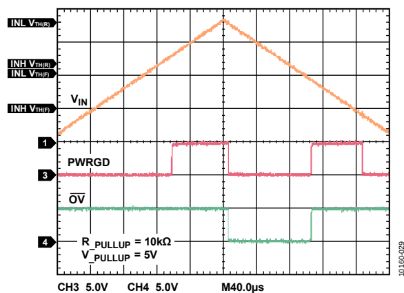
Figure 29. Propagation Delay
