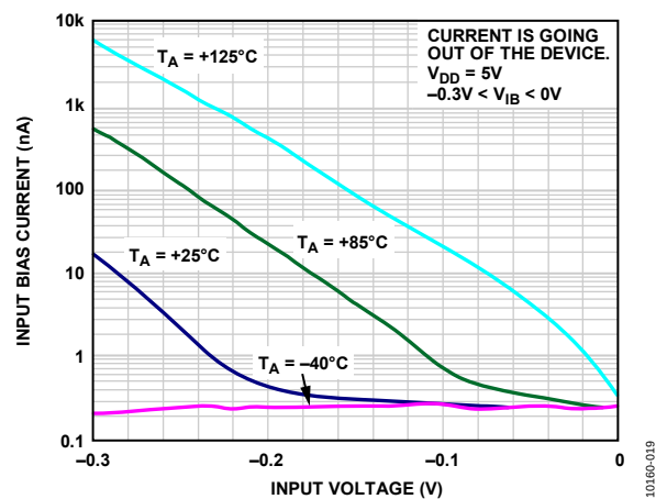
Figure 20. Below Ground Input Bias Current vs. Input Voltage
