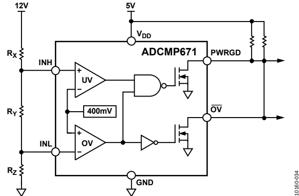
Figure 34. Undervoltage/Overvoltage Monitoring Configuration
