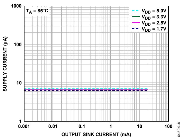
Figure 17. Supply Current vs. Output Sink Current for T_A = 85^\circ\text{C}
