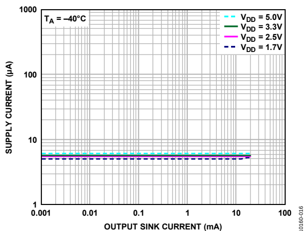
Figure 16. Supply Current vs. Output Sink Current for T_A = -40^\circ\text{C}
