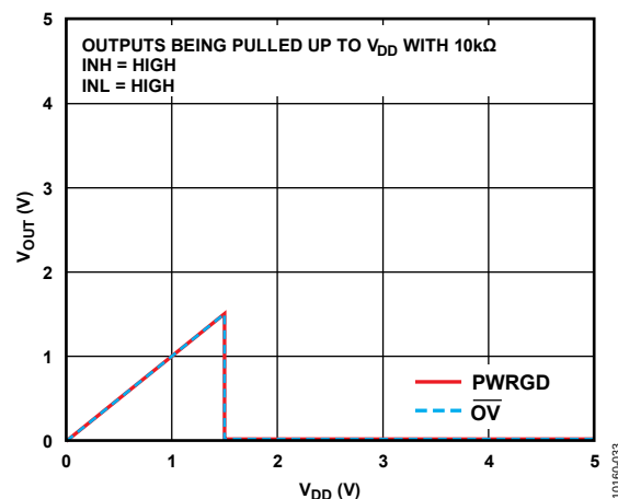
Figure 33. Output Voltage vs. Supply Voltage with Both INH and INL High
