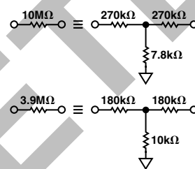
Figure 8. Equivalent Resistances
