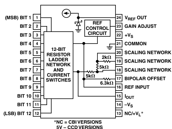
Figure 2. Current Model Functional Diagram and Pin Configuration
