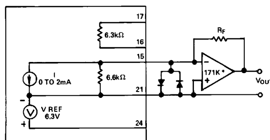
Figure 13. External Op Amp—Using External Feedback Resistors
