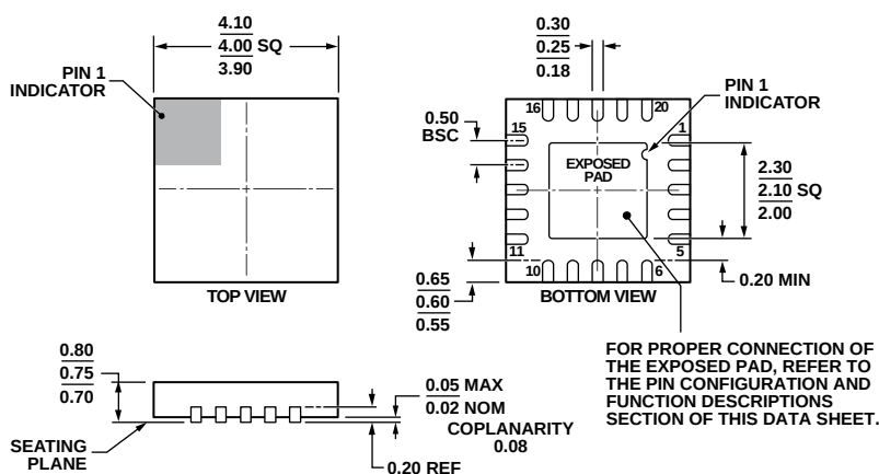
Figure 25. 20-Lead Lead Frame Chip Scale Package [LFCSP_WQ] 4mm × 4 mm Body, Very Very Thin Quad (CP-20-6)
