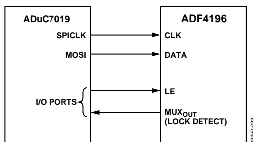
Figure 38. ADuC7019-to-ADF4196 Interface
