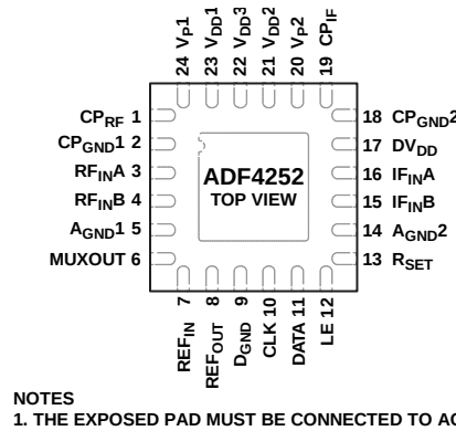
Figure 3. Pin Configuration
