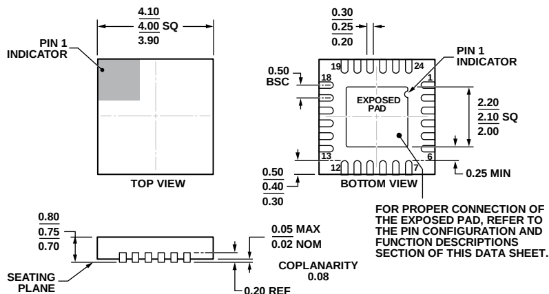
Figure 45. 24-Lead Lead Frame Chip Scale Package [LFCSP_WQ] 4 mm × 4 mm Body, Very Very Thin Quad (CP-24-10)
