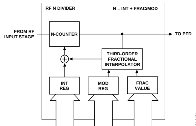
Figure 31. N Counter
