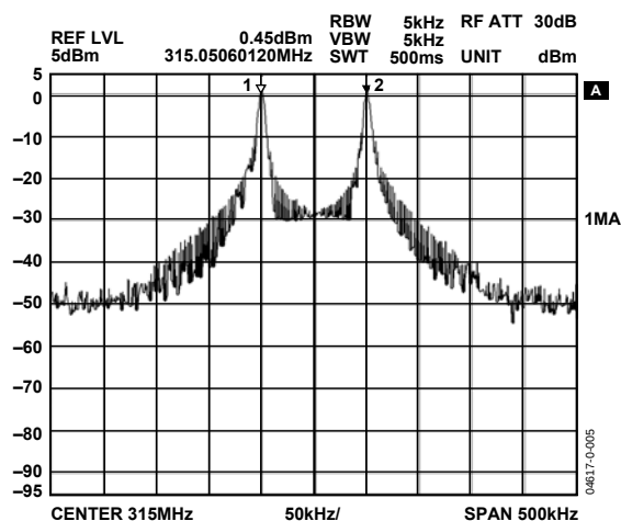
Figure 5. FSK Modulation, Power = 0 dBm, Data Rate = 1 kbps, F_{DEVIATION} = \pm 50\text{ kHz}
