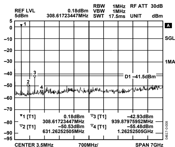
Figure 8. Harmonic Response, Fifth-Order Butterworth Filter
