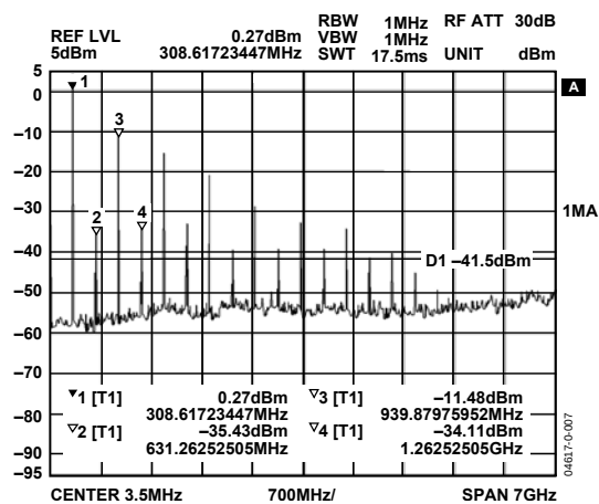
Figure 7. Harmonic Response, RF_{OUT} Matched to 50\ \Omega , No Filter
