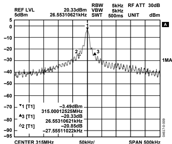
Figure 9. OOK Modulation, Power = 0 dBm, Data Rate = 10 kbps
