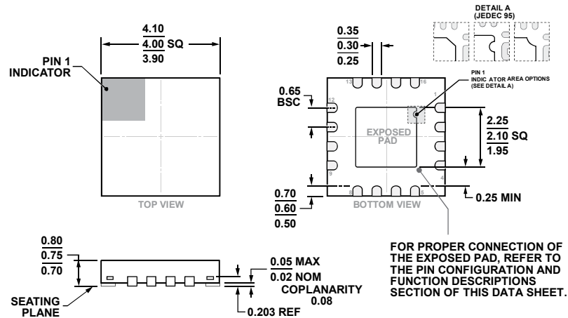
Figure 43. 16-Lead Lead Frame Chip Scale Package [LFCSP] 4 mm x 4 mm Body and 0.75 mm Package Height (CP-16-23)
