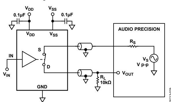
Figure 41. THD + N
