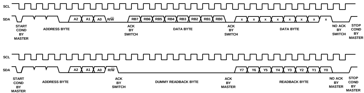
Figure 35. Read Operation
