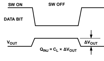
Figure 29. Charge Injection
