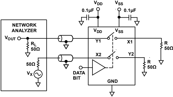
Figure 32. Channel-to-Channel Crosstalk
