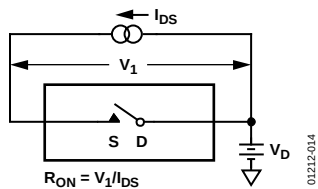
Figure 14. On Resistance
