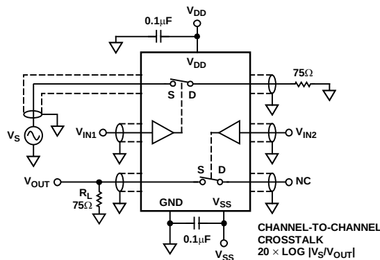
Figure 21. Channel-to-Channel Crosstalk
