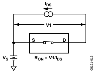
Figure 16. On Resistance
