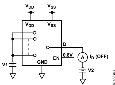
Figure 17. I_D (Off)
