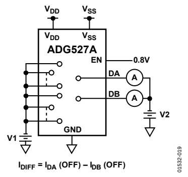
Figure 19. I_{DIFF}
