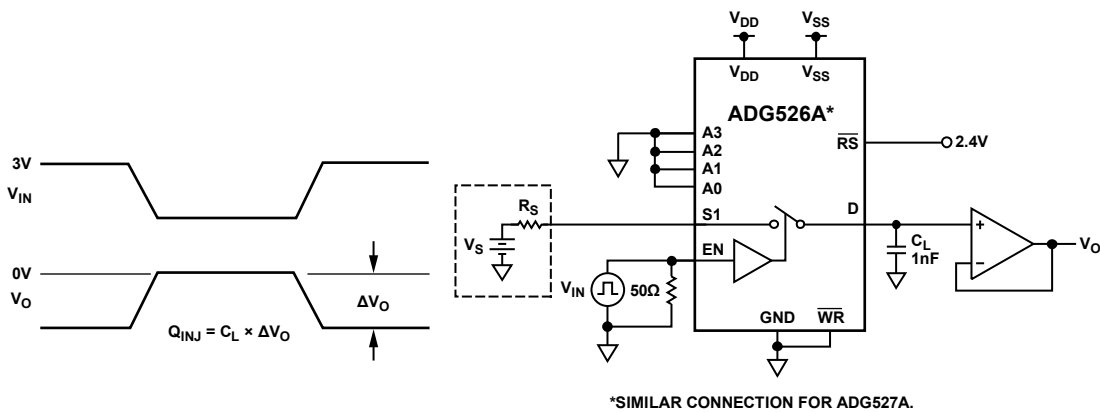
Figure 25. Charge Injection
