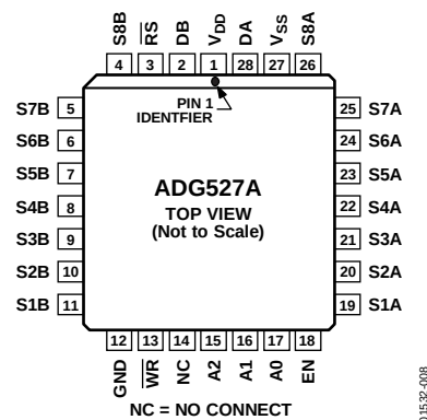
Figure 6. ADG527A PLCC Pin Configuration
