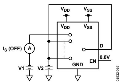
Figure 16. I_S (Off)
