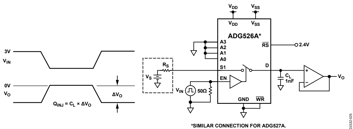
Figure 25. Charge Injection
