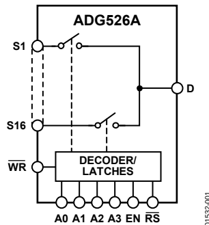
Figure 1. ADG526A
