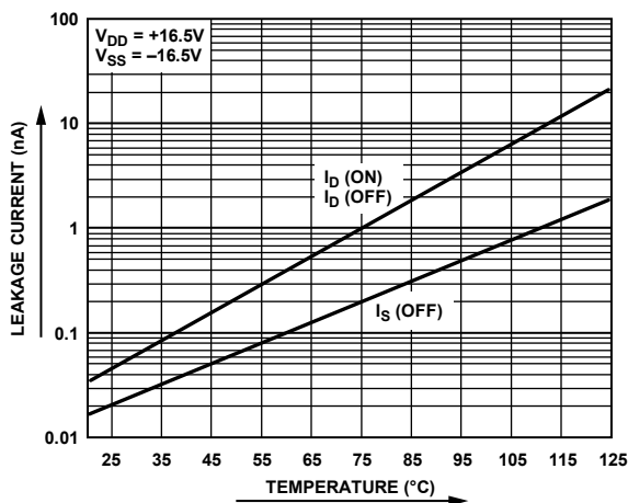
Figure 9. Leakage Current as a Function of Temperature (Leakage Currents Reduce as the Supply Voltages Reduce)
