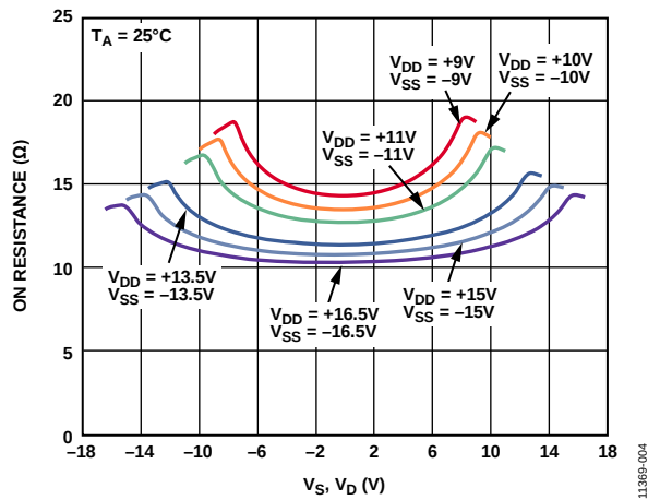
Figure 4. On Resistance as a Function of V_S , V_D (Dual Supply: \pm 10 V, \pm 15 V)
