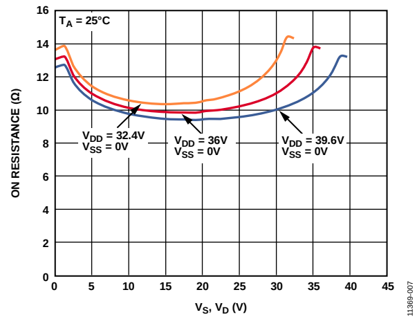
Figure 7. On Resistance as a Function of V_S , V_D (Single Supply: 36 V)
