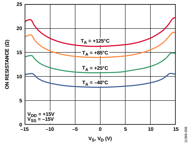
Figure 8. On Resistance as a Function of V_S ( V_D ) for Different Temperatures, \pm 15 V Dual Supply
