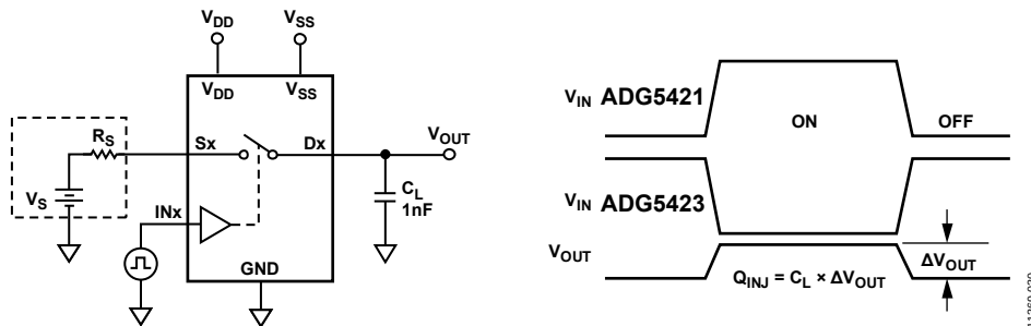
Figure 30. Charge Injection
