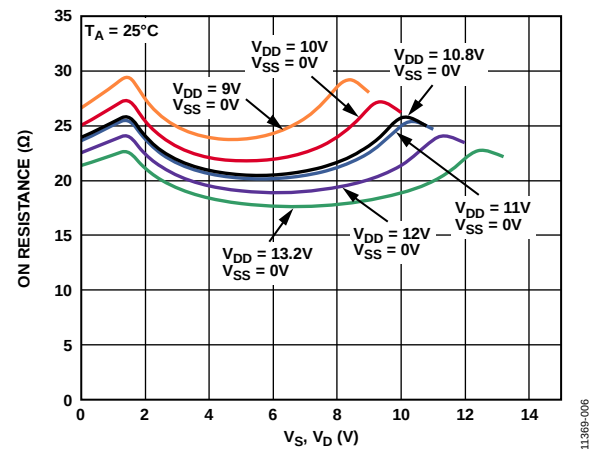
Figure 6. On Resistance as a Function of V_S , V_D (Single Supply: 10 V, 12 V)
