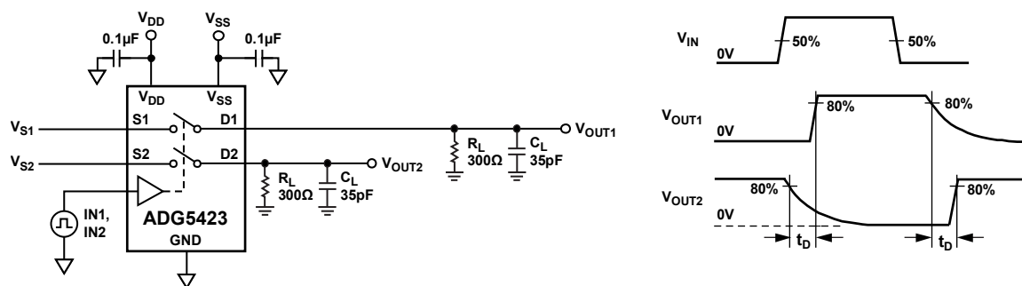
Figure 31. Break-Before-Make Time Delay
