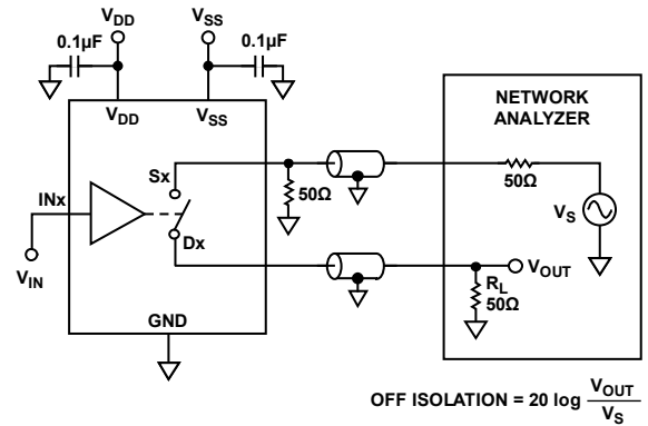
Figure 25. Off Isolation
