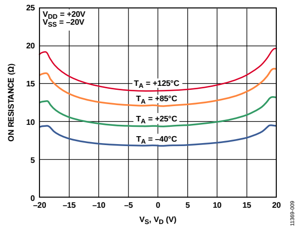
Figure 9. On Resistance as a Function of V_S ( V_D ) for Different Temperatures, \pm 20 V Dual Supply
