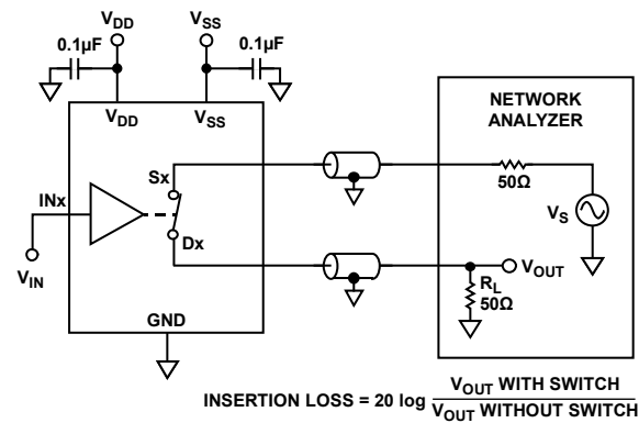
Figure 27. Bandwidth
