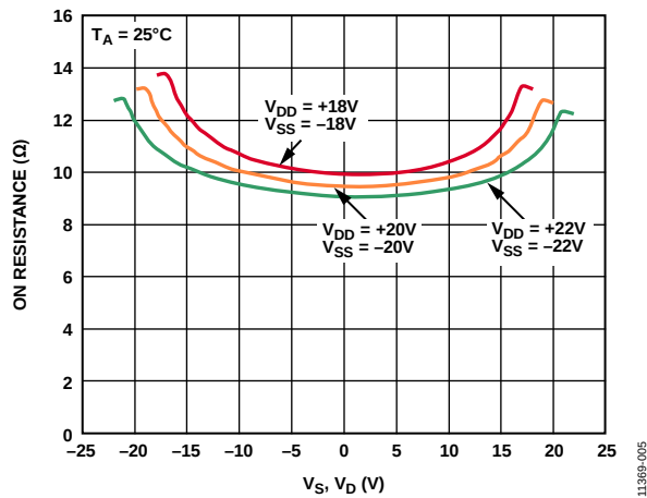
Figure 5. On Resistance as a Function of V_S , V_D (Dual Supply: \pm 20 V)
