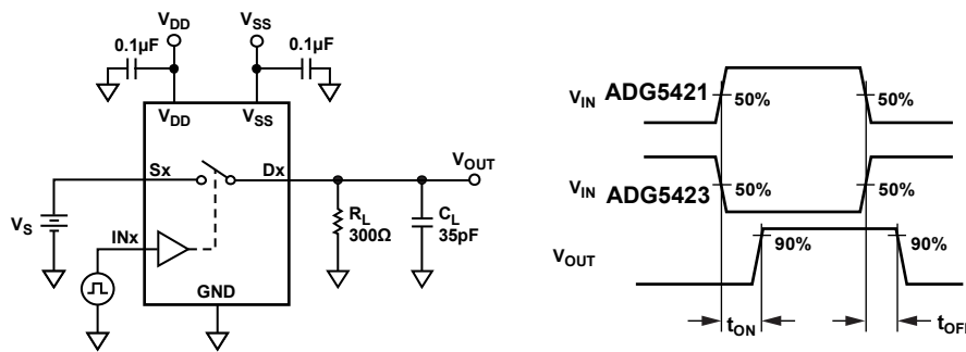
Figure 29. Switching Times, t_{ON} and t_{OFF}
