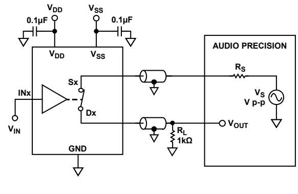
Figure 26. THD + Noise
