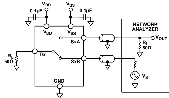
Figure 34. Channel-to-Channel Crosstalk
