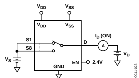
Figure 23. I_D (ON)
