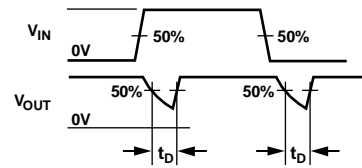
Figure 18. Break-Before-Make Time Delay, t_D
