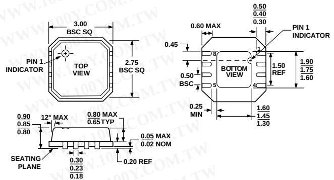
Figure 31. 8-Lead Lead Frame Chip Scale Package [LFCSP]
