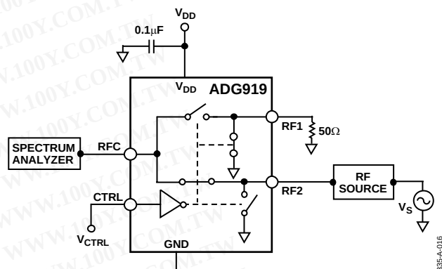
Figure 25. P 1dB
