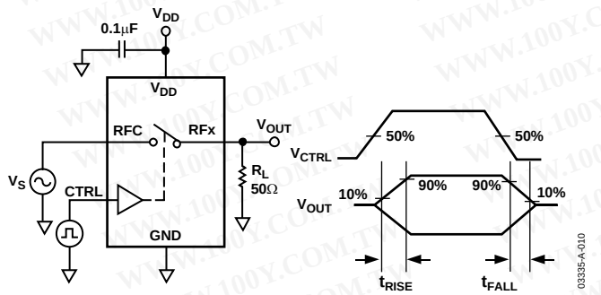
Figure 19. Switch Timing: t_{RISE} , t_{FALL}
