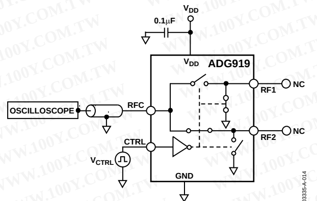
Figure 23. Video Feedthrough
