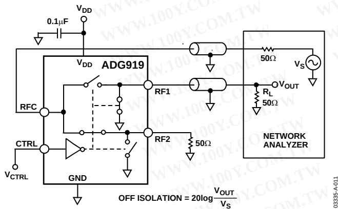
Figure 20. Off Isolation
