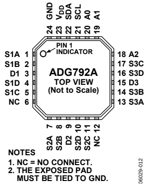
Figure 3. ADG792A Pin Configuration
