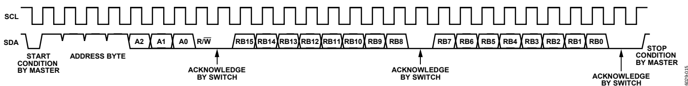
Figure 32. Read Operation
