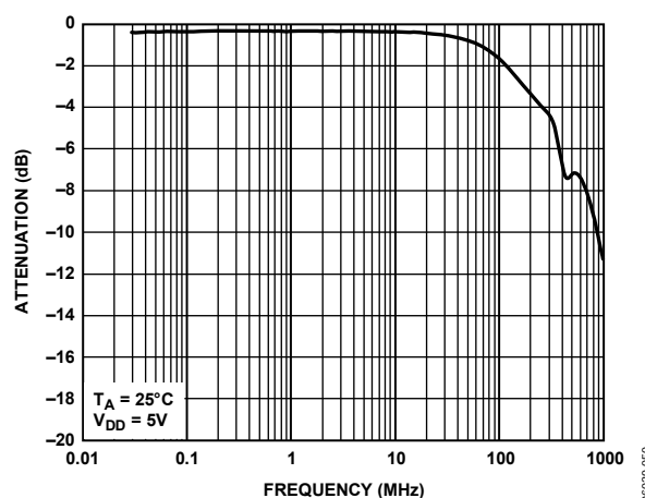
Figure 15. Bandwidth
