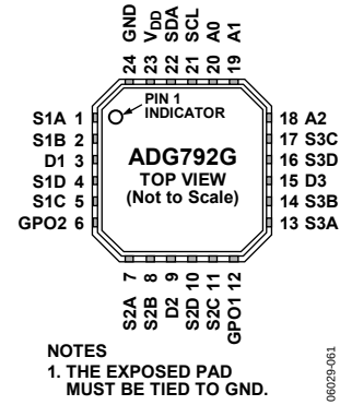
Figure 4. ADG792G Pin Configuration
