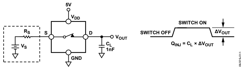
Figure 30. Charge Injection
