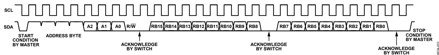
Figure 32. ADG795A/ADG795G Read Operation
