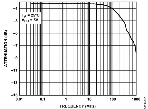
Figure 15. Bandwidth
