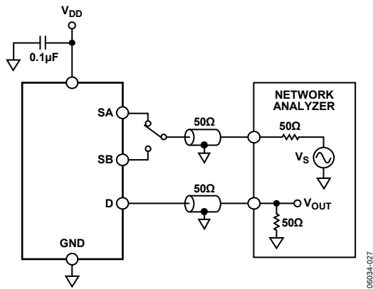
Figure 25. Bandwidth
