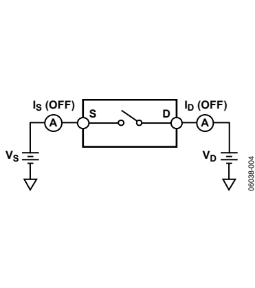
Figure 23. Off Leakage
