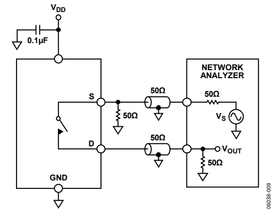
Figure 26. Off Isolation
