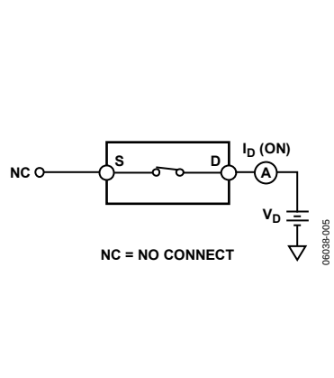
Figure 24. On Leakage
