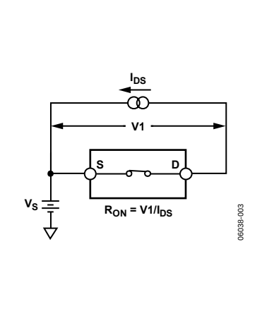
Figure 22. On Resistance
