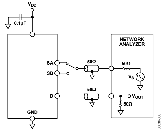
Figure 25. Bandwidth
