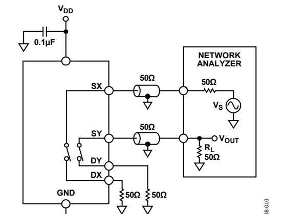
Figure 27. Channel-to-Channel Crosstalk
