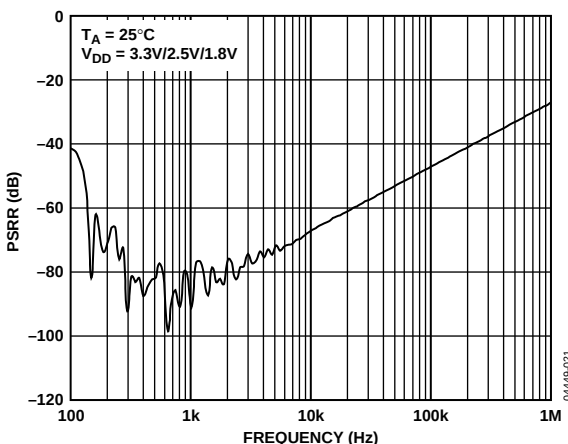
Figure 18. AC PSRR
