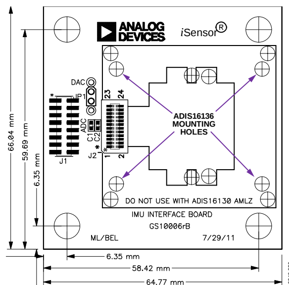
Figure 22. Physical Diagram for the ADIS16136IMU1/PCBZ
