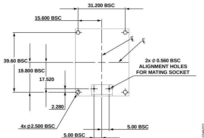
Figure 24. Suggested Mounting Hole Locations, Connector Down
