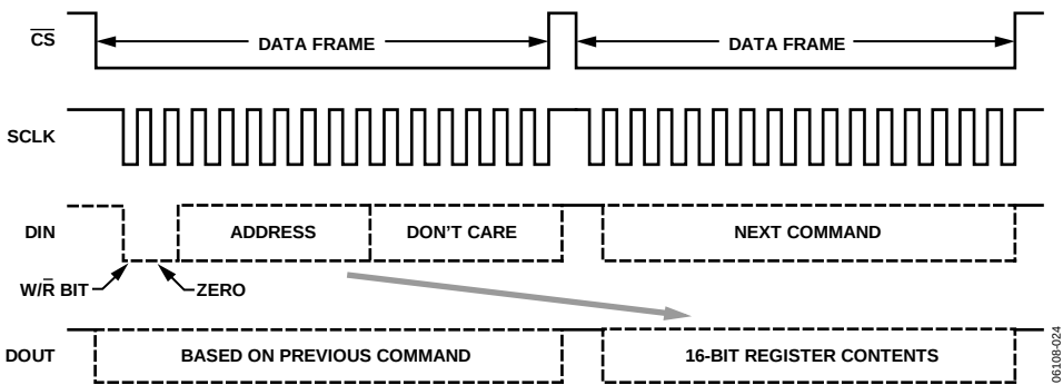
Figure 27. SPI Sequence for Read Commands
