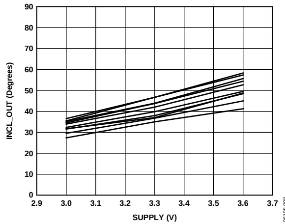
Figure 8. Self-Test Shift vs. Supply at 25°C
