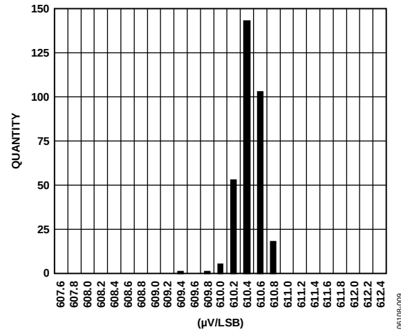
Figure 9. ADC Gain Distribution at 25°C/3.3 V
