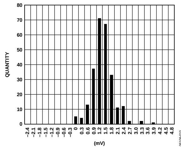
Figure 10. ADC Offset Distribution at 25°C/3.3 V
