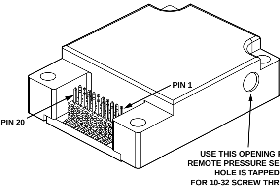
Figure 6. Pin Locations
