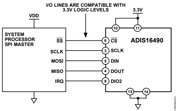
Figure 29. Electrical Connection Diagram
