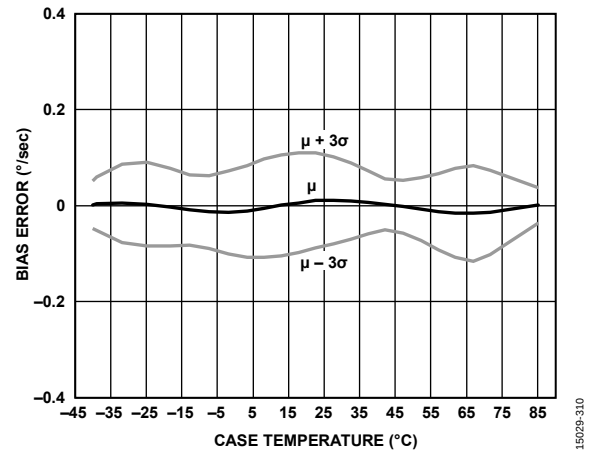
Figure 10. Gyroscope Bias Error, -40°C to +85°C, 1°C/min
