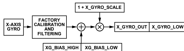
Figure 43. User Calibration Signal Path, Gyroscopes
