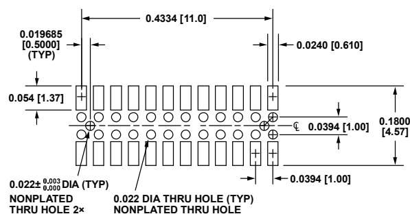
Figure 49. Suggested Layout and Mechanical Design When Using Samtec CLM-112-02-G-D-A for the Mating Connector
