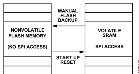
Figure 34. SRAM and Flash Memory Diagram
