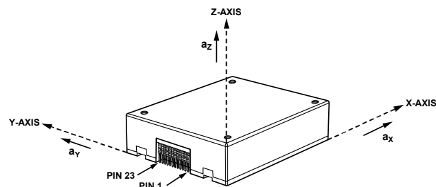
Figure 37. Accelerometer Axis and Polarity Assignments
