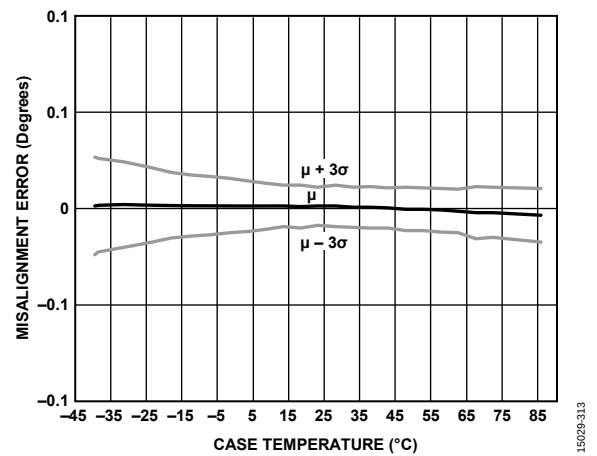
Figure 11. Gyroscope Axis to Axis Misalignment Error, -40°C to +85°C
