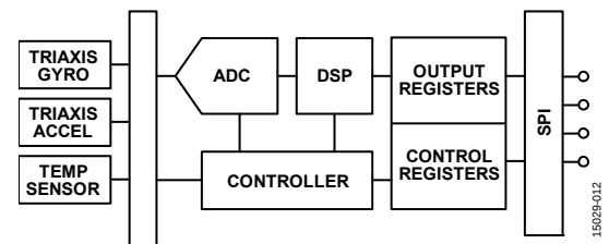
Figure 27. Basic Operation
