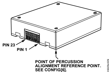
Figure 46. Point of Percussion Reference Point
