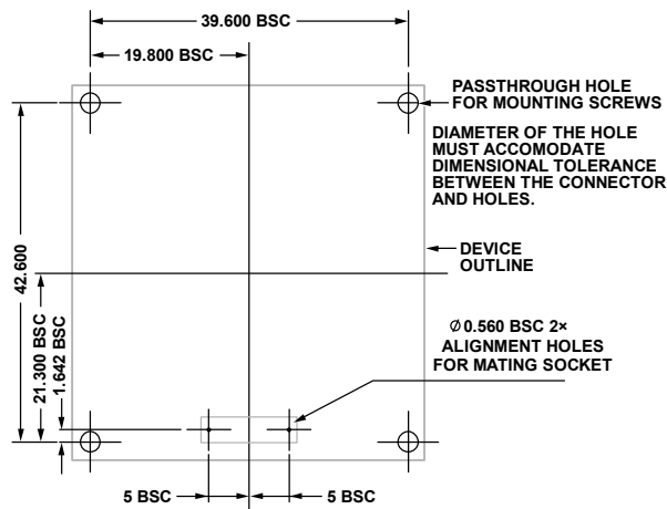
Figure 48. Suggested PCB Layout Pattern, Connector Down
