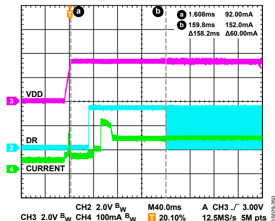
Figure 50. Transient Current Demand, Startup (DR Means Data Ready)
