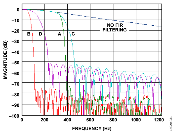
Figure 47. FIR Filter Frequency Response Curves
