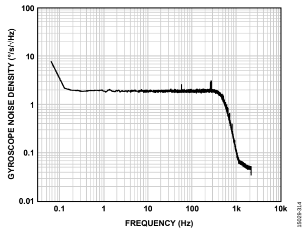
Figure 12. Gyroscope Noise Density, T_c = 25^\circ\text{C}
