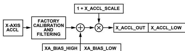
Figure 44. User Calibration Signal Path, Accelerometers
