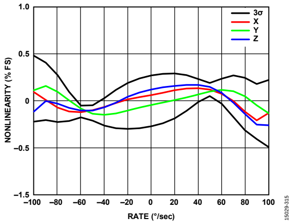
Figure 13. Gyroscope Nonlinearity
