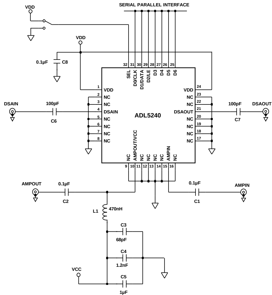
Figure 34. Basic Connections
