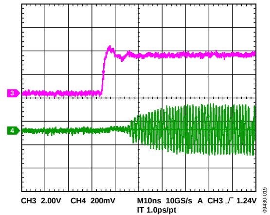
Figure 19. DSA: Gain Settling Time, 31.5 dB to 0 dB
