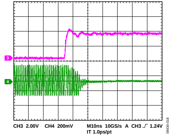
Figure 18. DSA: Gain Settling Time, 0 dB to 31.5 dB
