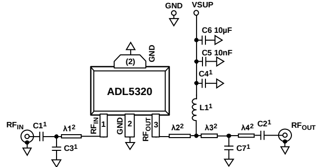
Figure 34. Basic Connections
