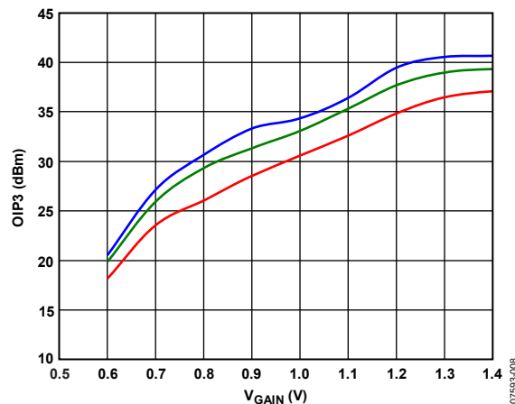
Figure 8. Output IP3 vs. V_{\text{GAIN}} at 400 MHz
