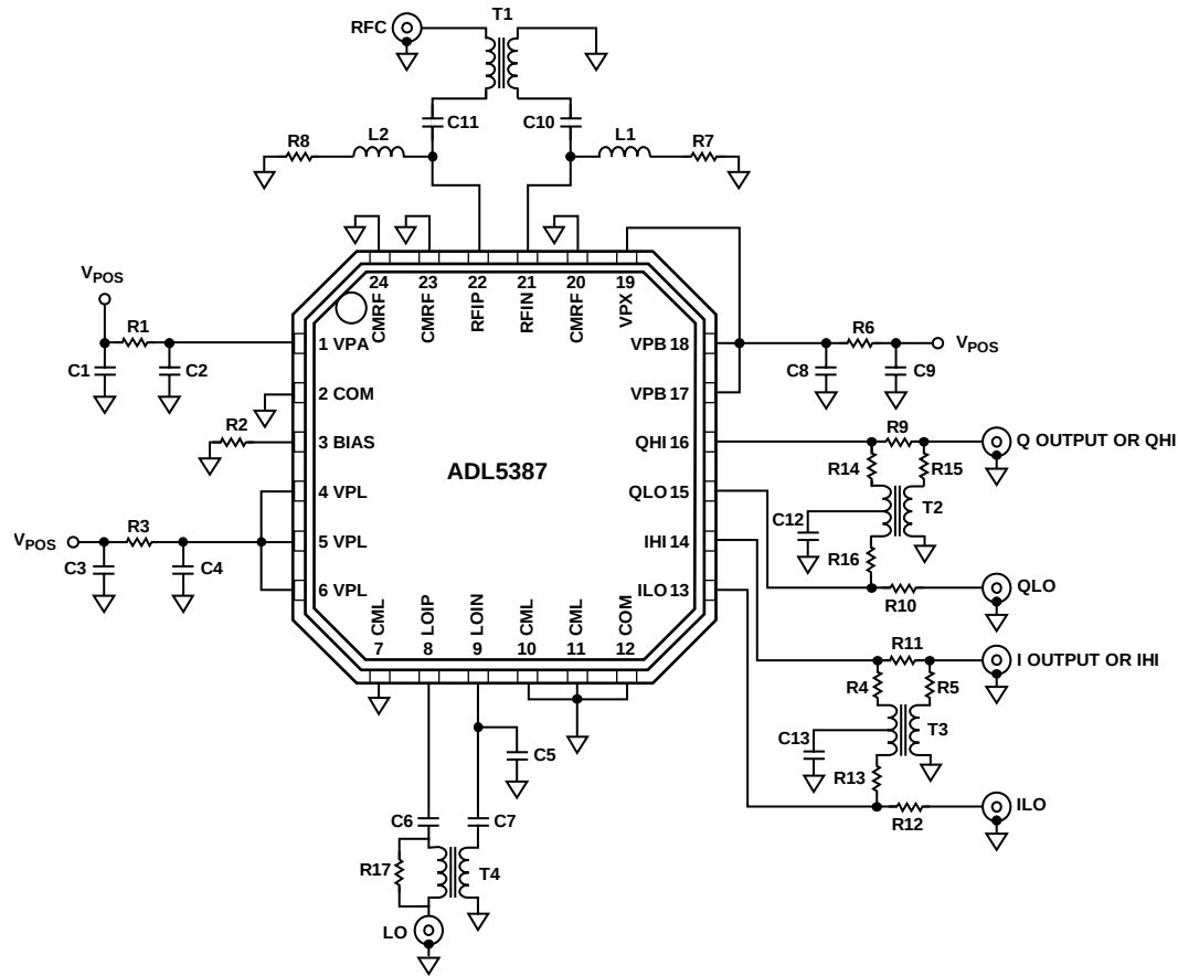
Figure 67. Evaluation Board Schematic
