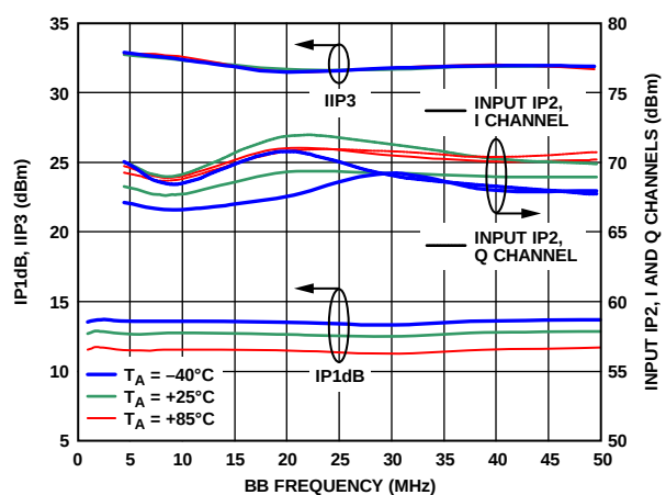
Figure 19. IIP3, IIP2, IP1dB vs. Baseband Frequency
