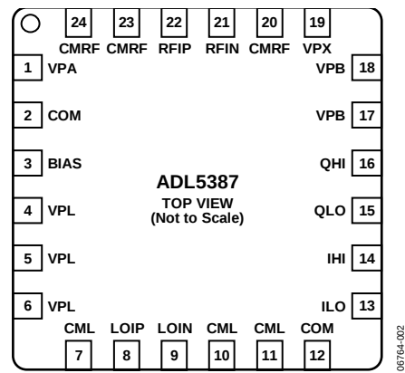
Figure 2. Pin Configuration
