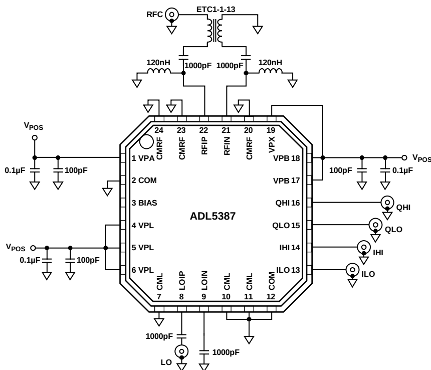
Figure 51. Basic Connections Schematic for ADL5387
