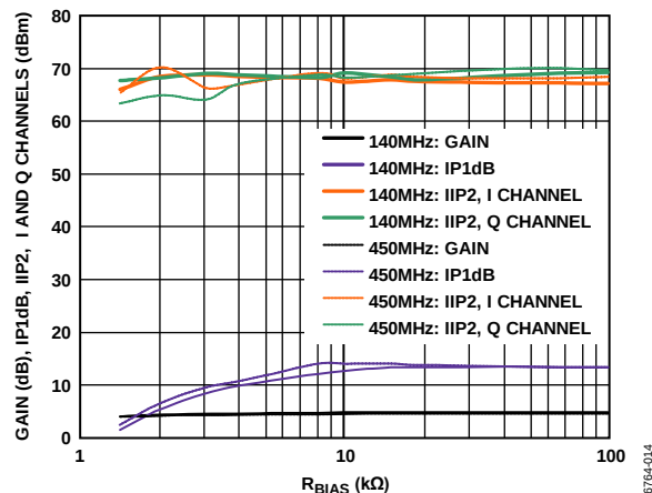
Figure 18. Conversion Gain, IP1dB, IIP2, I and IIP2 Q Channel vs. R_{BIAS}
