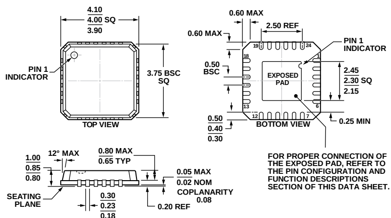
Figure 72. 24-Lead Lead Frame Chip Scale Package [LFCSP_VQ] 4 mm × 4 mm Body, Very Thin Quad (CP-24-2) Dimensions shown in millimeters
