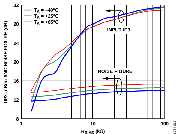
Figure 17. IIP3 and Noise Figure vs. R_{BIAS} , f_{RF} = 900 MHz
