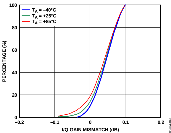
Figure 45. I/Q Gain Mismatch Distributions
