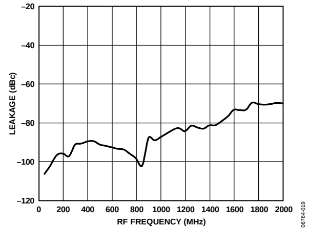
Figure 23. RF-to-LO Leakage vs. RF Frequency
