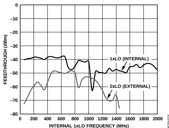
Figure 20. LO-to-BB Feedthrough vs. 1xLO Frequency (Internal LO Frequency)
