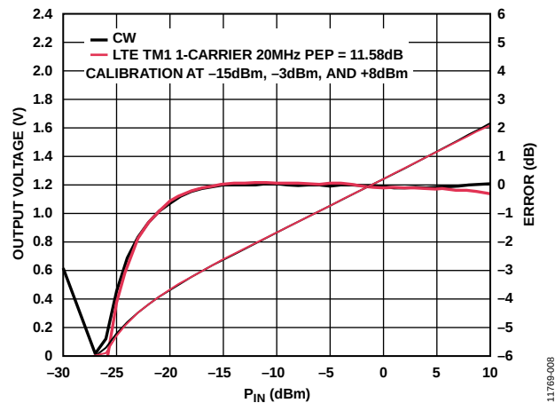
Figure 8. Error from CW Linear Reference vs. Input Level and Signal Modulation (LTE TM1 One-Carrier, 20 MHz), Frequency = 2.14 GHz, C_{RMS} = 1 \mu F
