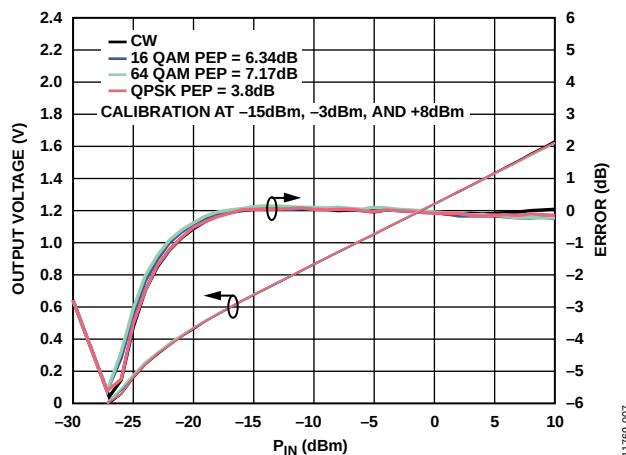
Figure 7. Error from CW Linear Reference vs. Input Level and Signal Modulation (QPSK, 16 QAM, 64 QAM), Frequency = 2.14 GHz, C_{RMS} = 1 \mu F
