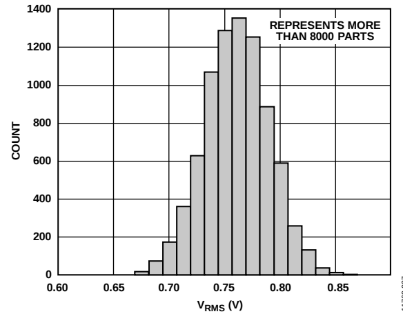
Figure 32. Distribution of V_{RMS} , P_{IN} = -16 \text{ dBm} , 900 MHz
