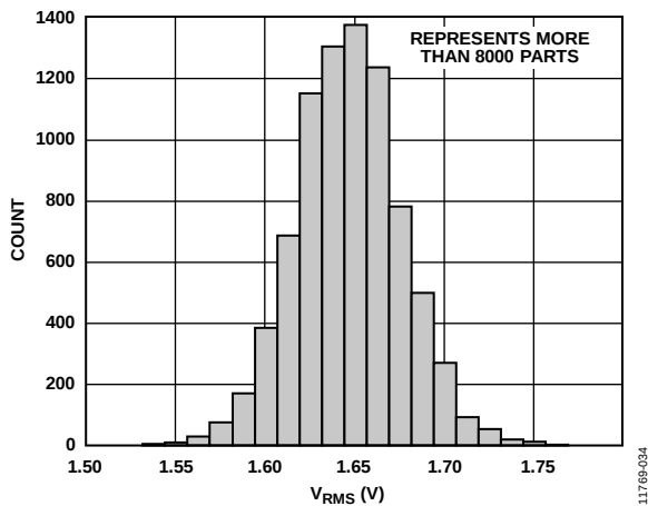
Figure 29. Distribution of V_{RMS} , P_{IN} = 8 \text{ dBm} , 900 MHz
