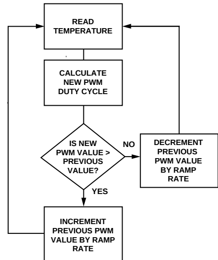
Figure 29. Filtered Mode Algorithm
