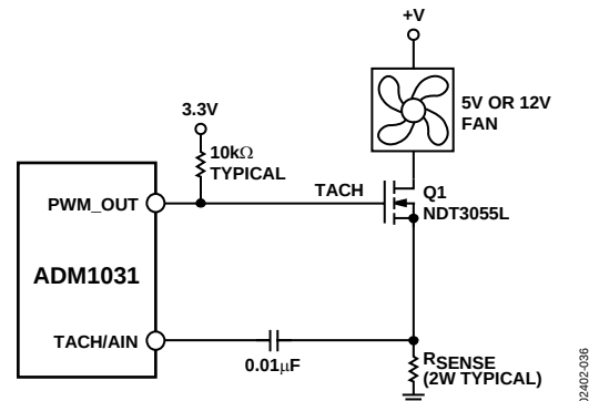
Figure 36. Interfacing the ADM1031 to a 2-Wire Fan
