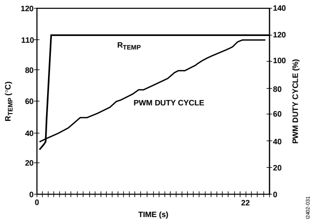
Figure 31. Filtered Mode with Ramp Rate = 4
