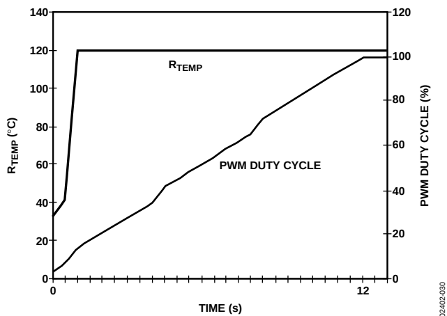
Figure 30. Filtered Mode with Ramp Rate = 8
