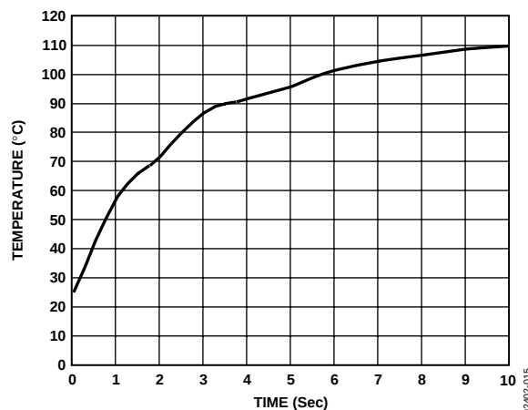
Figure 15. Response to Thermal Shock
