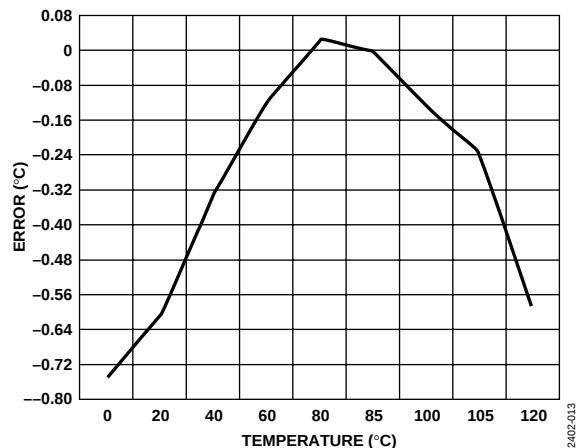
Figure 13. Remote Temperature Sensor Error
