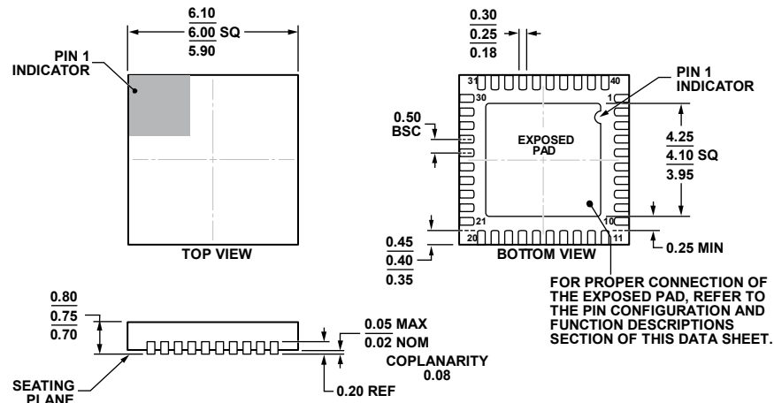
Figure 46. 40-Lead Lead Frame Chip Scale Package [LFCSP_WQ] 6 mm × 6 mm Body, Very Very Thin Quad (CP-40-9) Dimensions shown in millimeters
