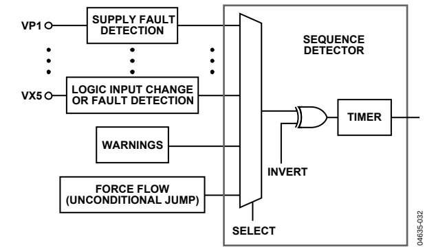
Figure 24. Sequence Detector Block Diagram
