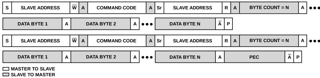
Figure 62. Block Read and Block Read with PEC
