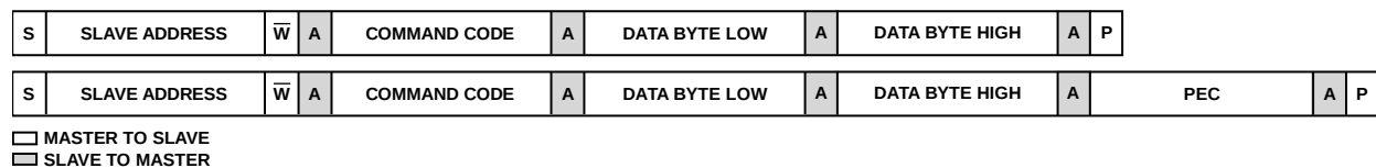
Figure 60. Write Word and Write Word with PEC
