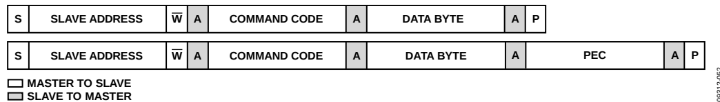
Figure 58. Write Byte and Write Byte with PEC
