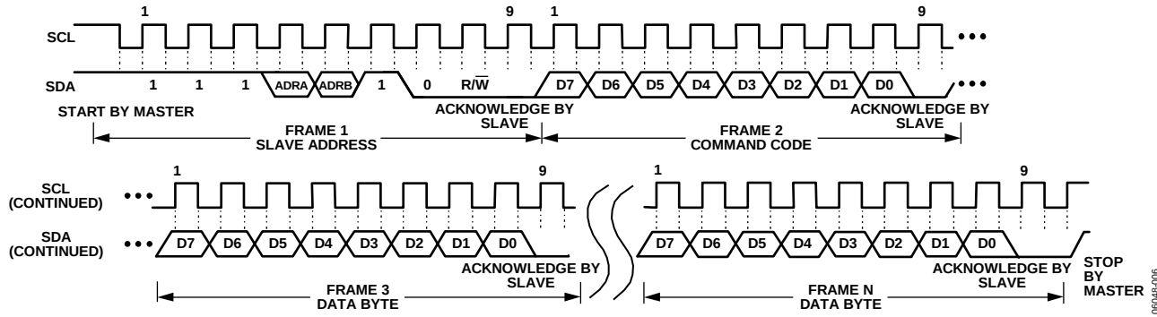
Figure 35. General I²C Write Timing Diagram
