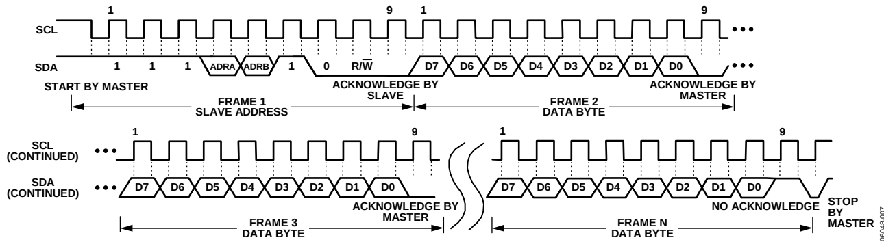
Figure 36. General I²C Read Timing Diagram
