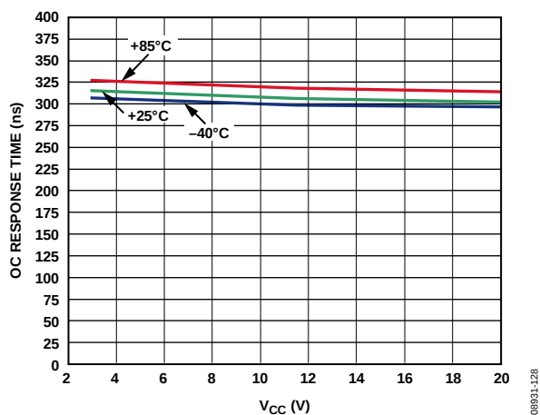
Figure 27. Severe Overcurrent Response Time vs. Supply Voltage ( V_{CC} ), V_{ISET} = 0.25 V
