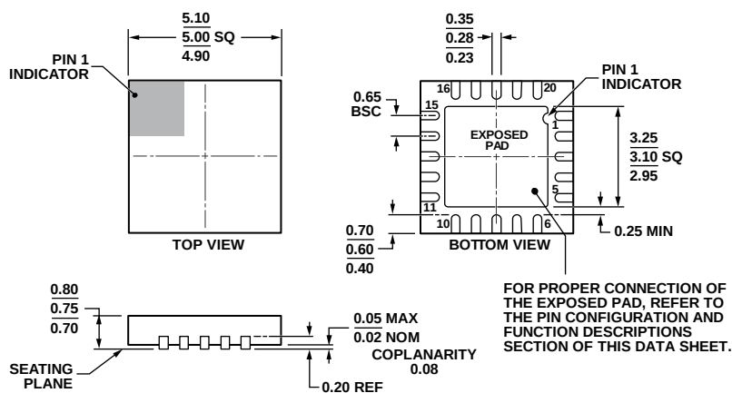
Figure 68. 20-Lead Lead Frame Chip Scale Package [LFCSP_WQ] 5 mm × 5 mm Body, Very Very Thin Quad (CP-20-9)
