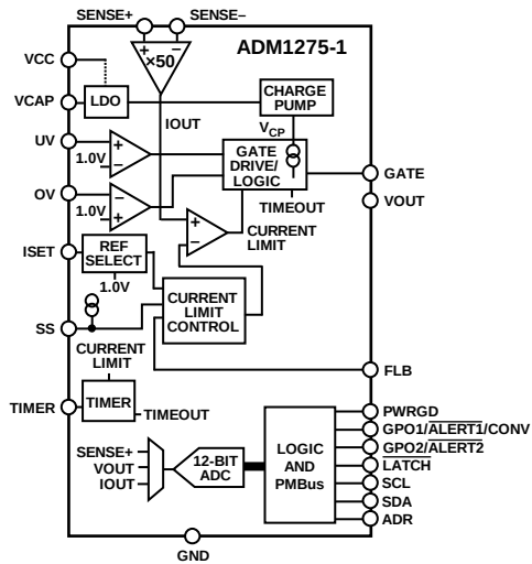
Figure 43. ADM1275-1 Functional Block Diagram
