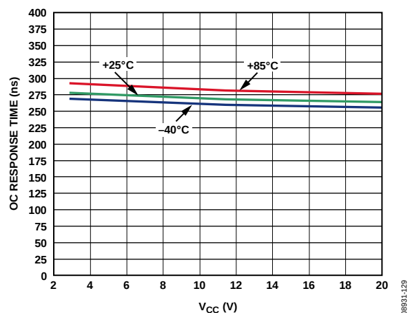
Figure 28. Severe Overcurrent Response Time vs. Supply Voltage ( V_{CC} ), V_{ISET} = 1 V
