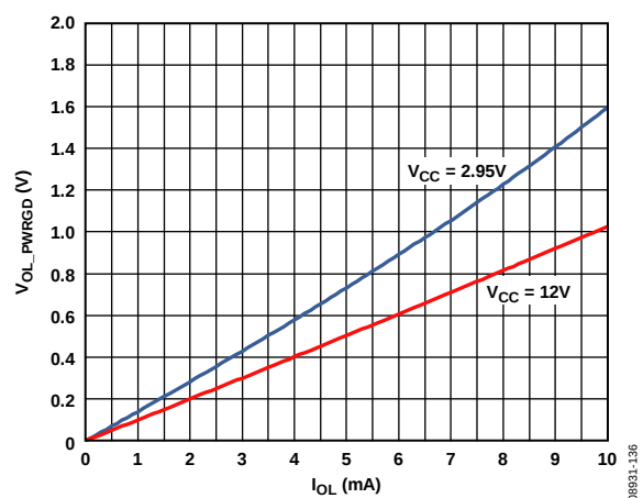
Figure 36. PWRGD Pin, V_{OL\_PWRGD} vs. I_{OL}
