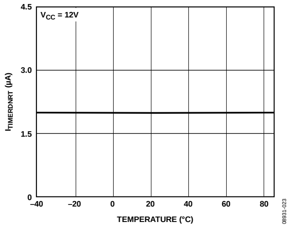
Figure 22. Timer Pull-Down Current, Retry ( I_{\text{TIMERDNRT}} ) vs. Temperature
