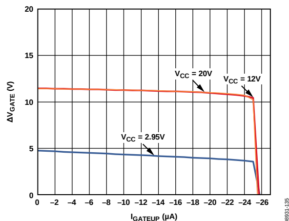
Figure 35. Gate Drive Voltage ( \Delta V_{GATE} ) vs. Gate Pull-Up Current ( I_{GATEUP} )
