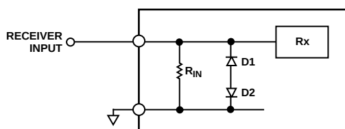
Figure 22a. Receiver Input Protection Scheme
