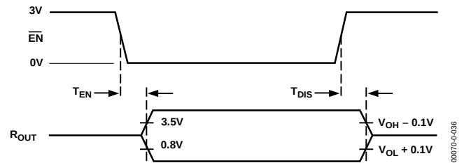
Figure 31. Enable Timing
