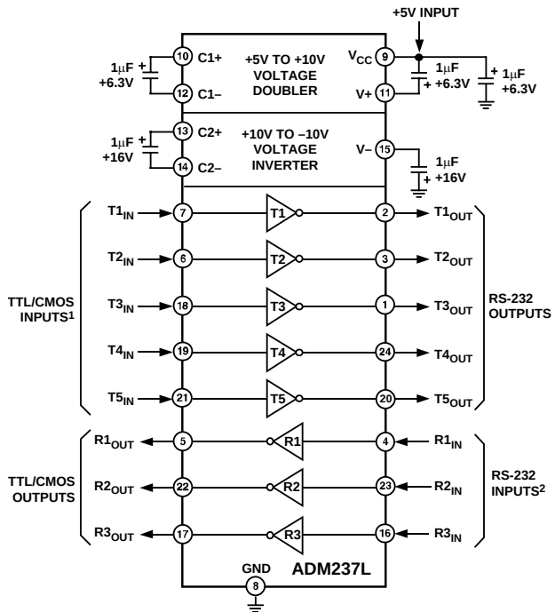
Figure 22. ADM237L Typical Operating Circuit
