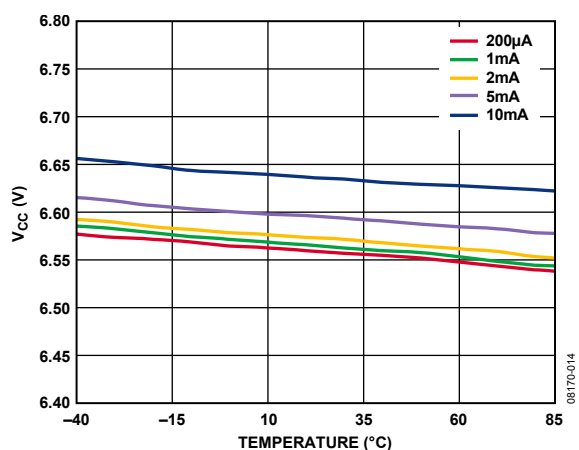
Figure 6. V_{CC} Shunt Voltage vs. Temperature
